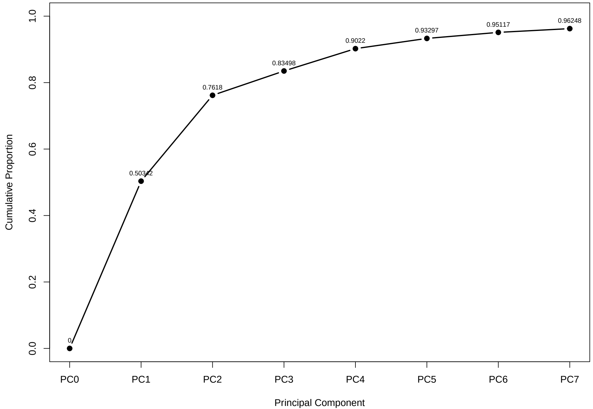
Scree Plot
